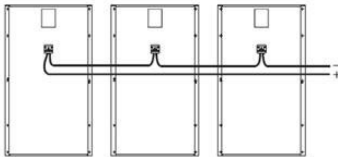
Series wiring
